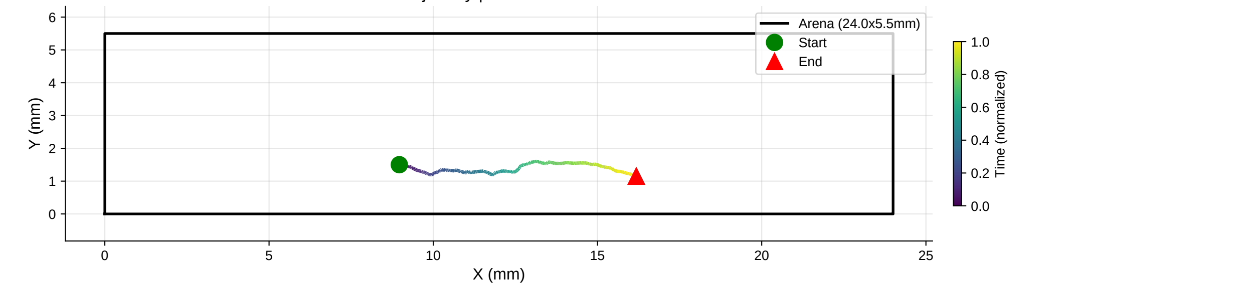
XY Trajectory | Distance: 7.87 mm
