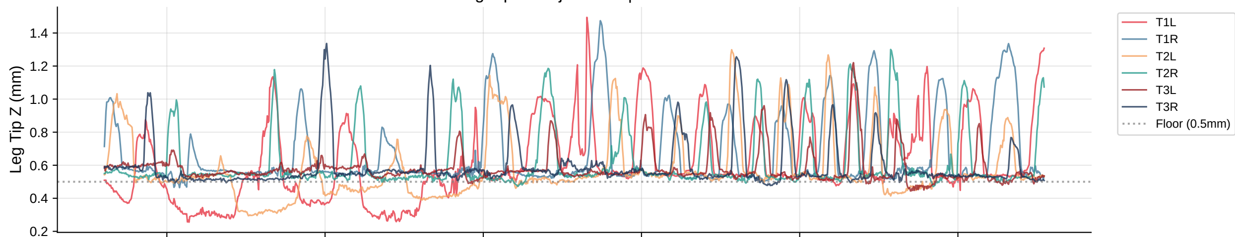
Leg Tip Z Trajectories | Bout 70
