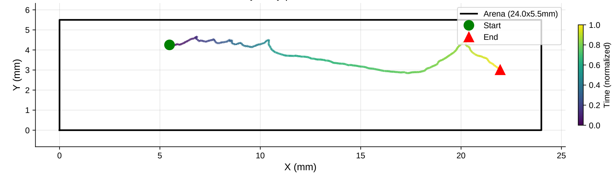
XY Trajectory | Distance: 20.58 mm
