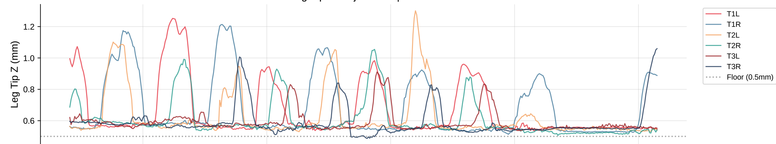
Leg Tip Z Trajectories | Bout 71
