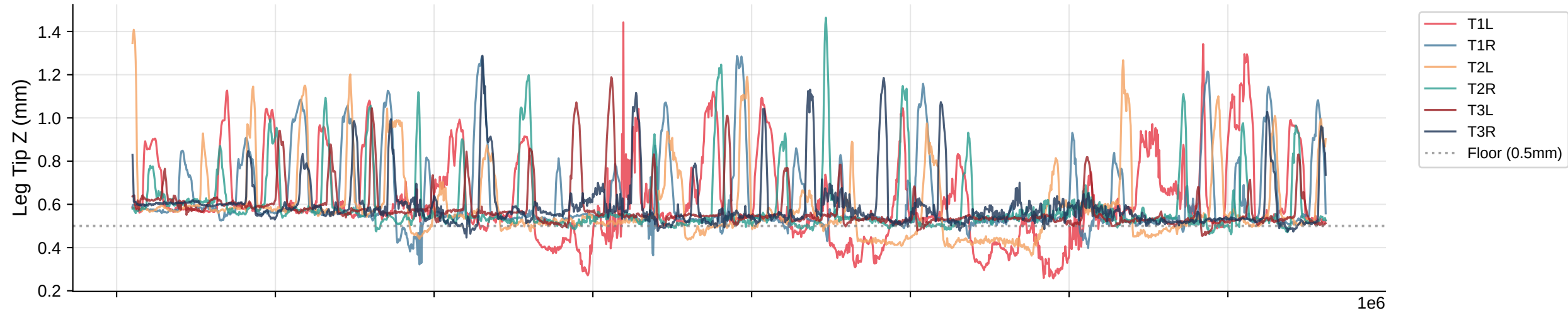
Leg Tip Z Trajectories | Bout 72
