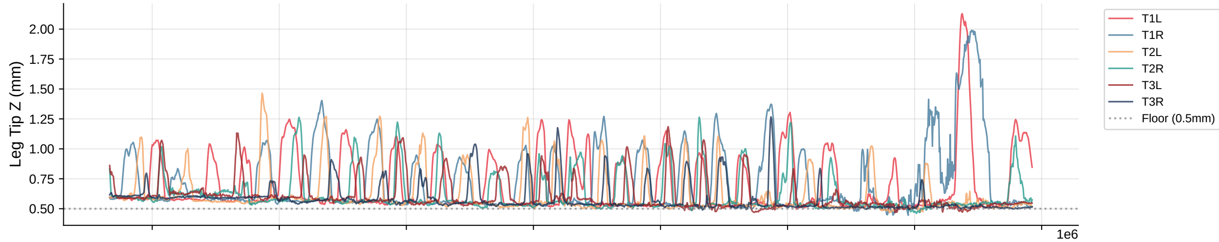
Leg Tip Z Trajectories | Bout 78
