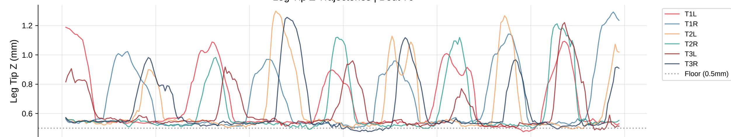
Leg Tip Z Trajectories | Bout 79
