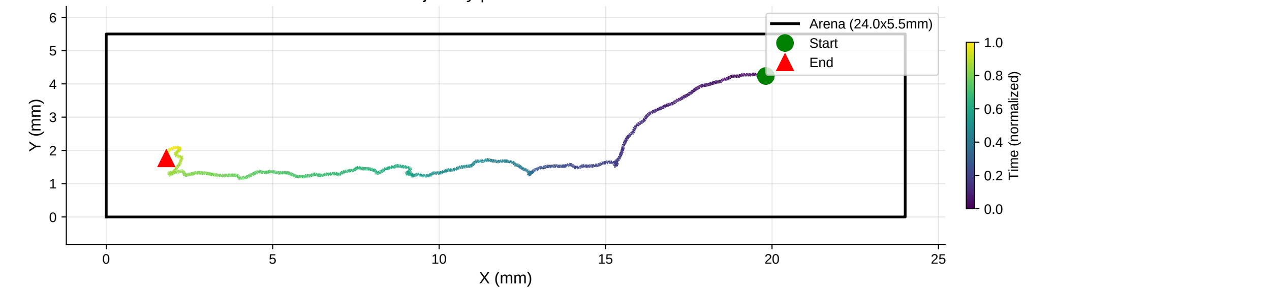
XY Trajectory | Distance: 26.91 mm
