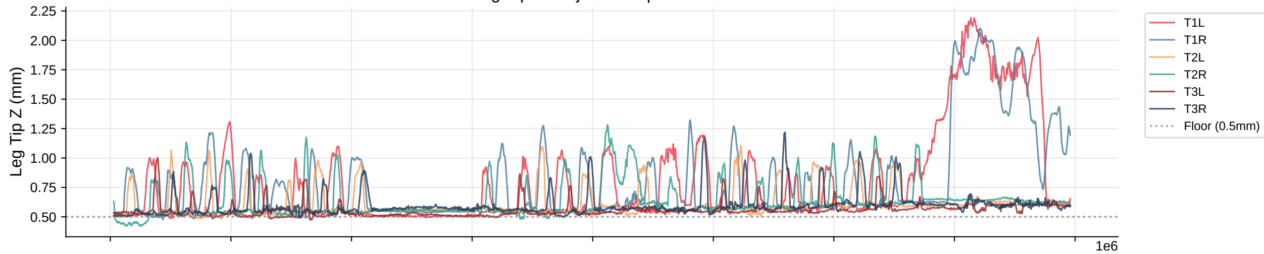
Leg Tip Z Trajectories | Bout 90
