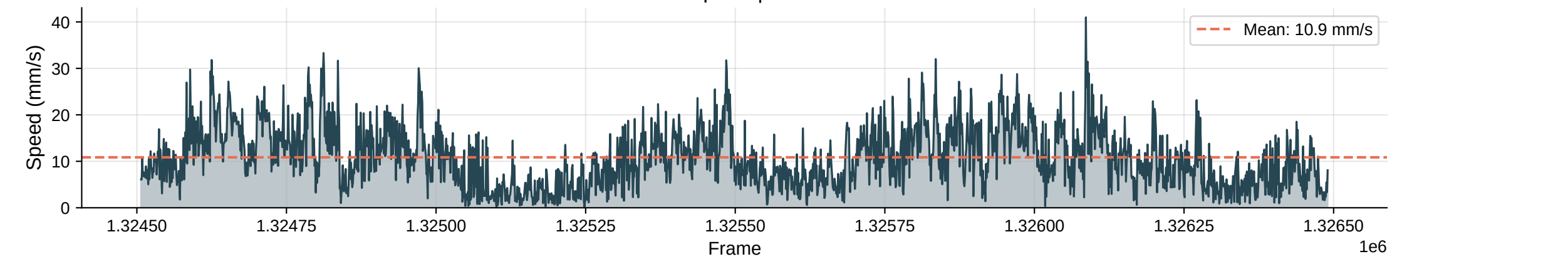
Instantaneous Speed | Max: 41.0 mm/s
