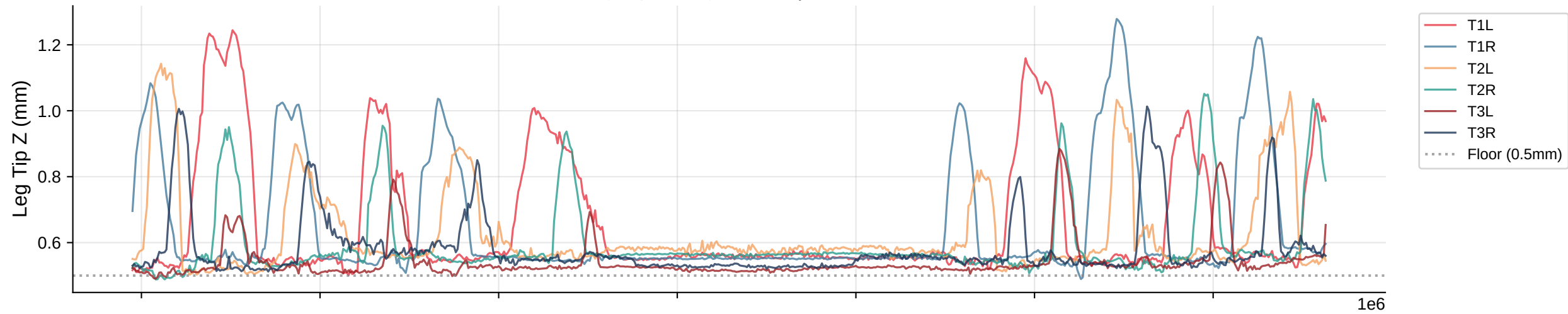
Leg Tip Z Trajectories | Bout 93
