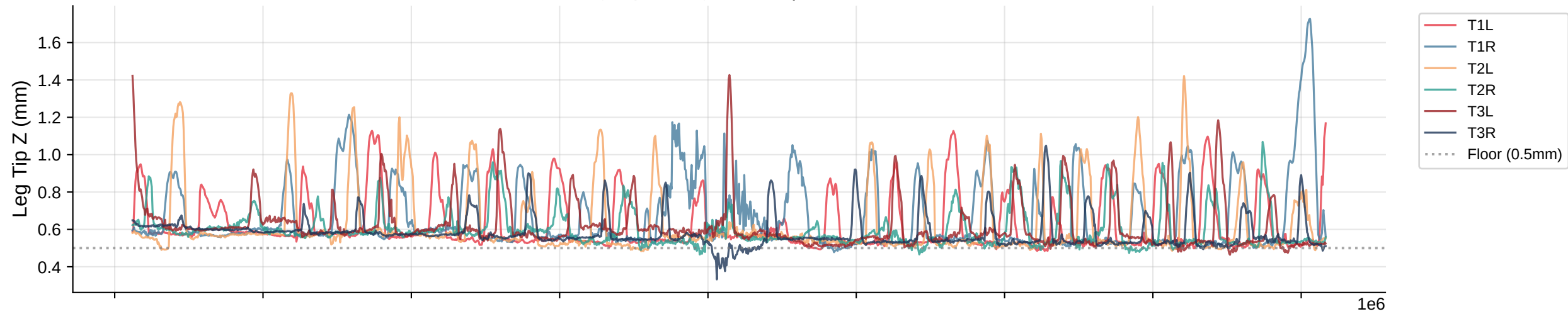
Leg Tip Z Trajectories | Bout 105
