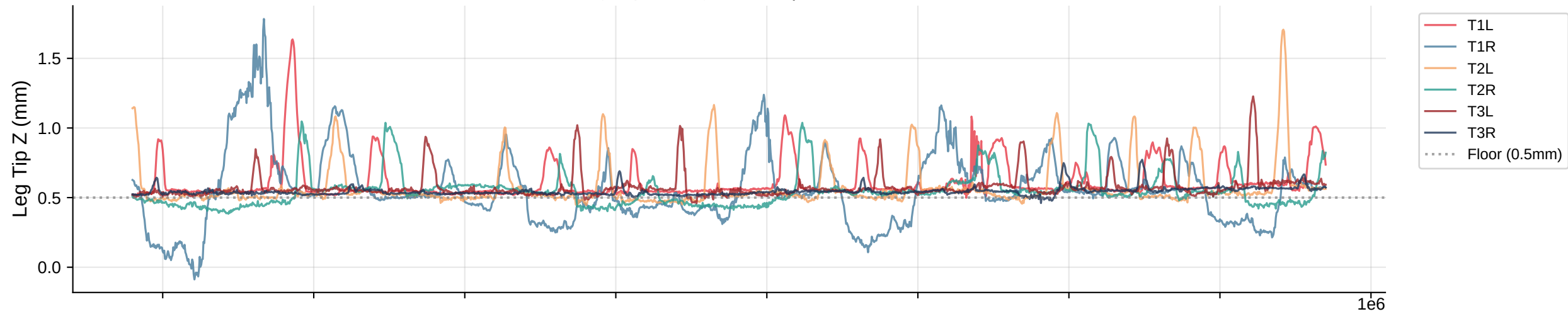
Leg Tip Z Trajectories | Bout 106
