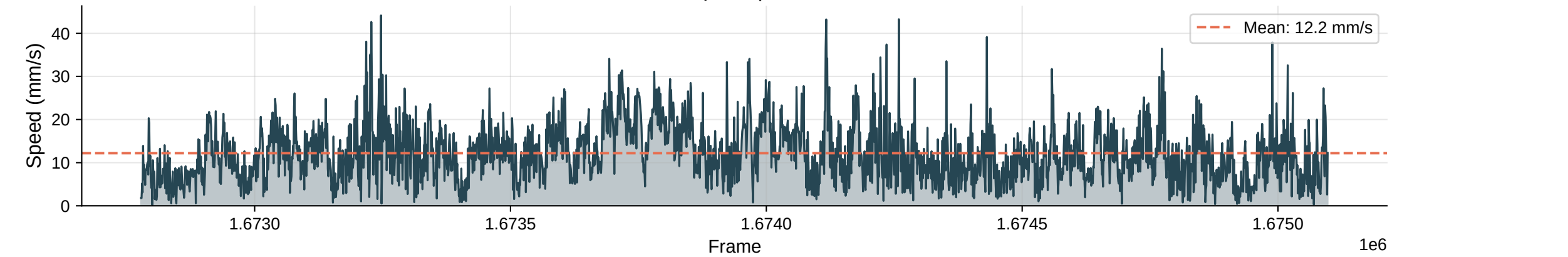
Instantaneous Speed | Max: 44.1 mm/s
