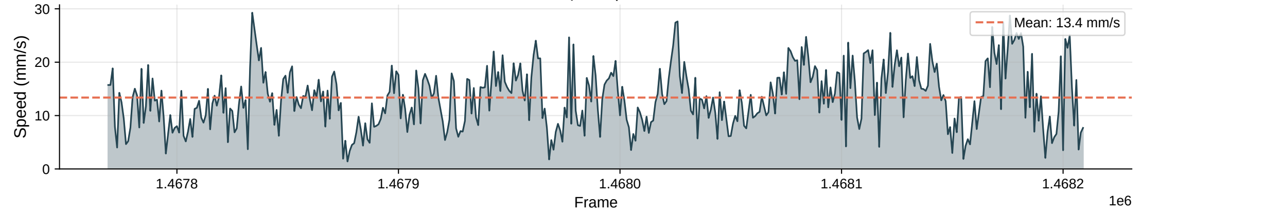
Instantaneous Speed | Max: 29.3 mm/s
