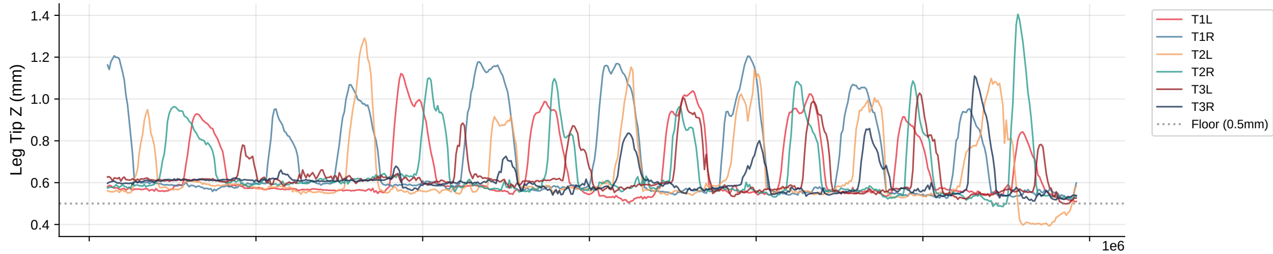
Leg Tip Z Trajectories | Bout 119
