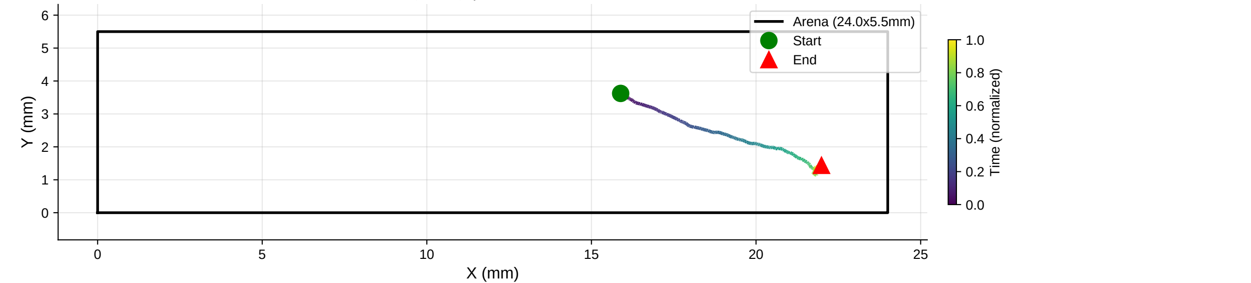
XY Trajectory | Distance: 7.66 mm
