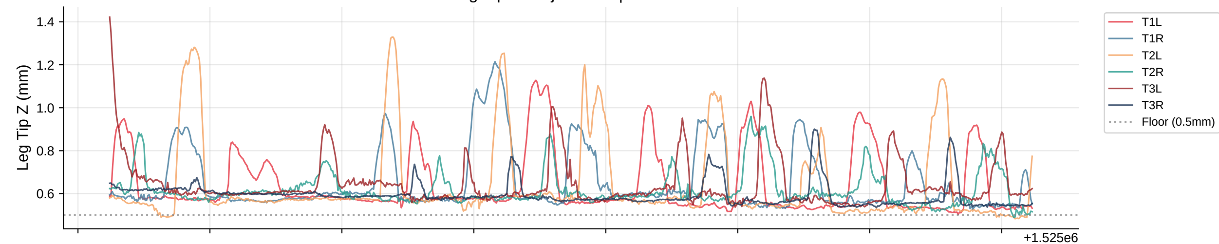
Leg Tip Z Trajectories | Bout 121
