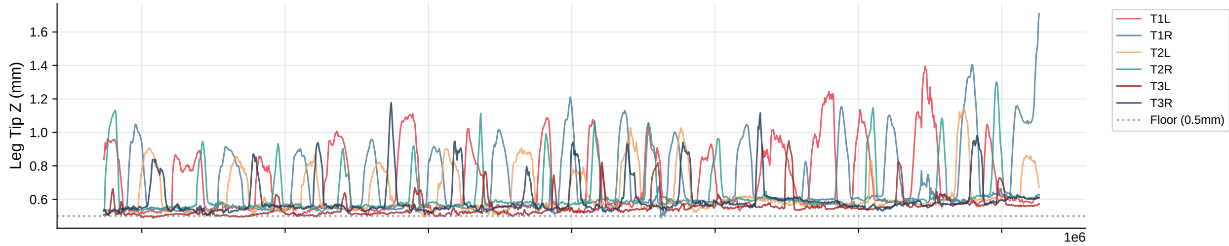
Leg Tip Z Trajectories | Bout 123
