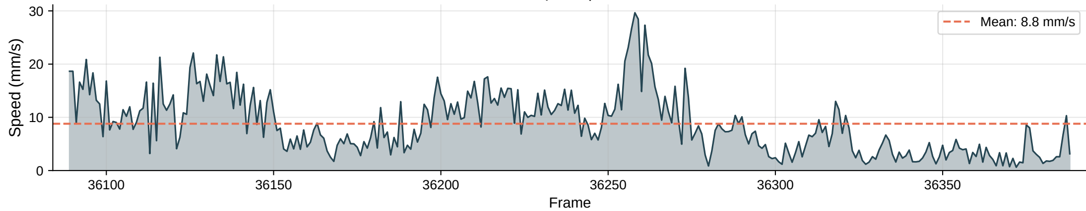
Instantaneous Speed | Max: 29.7 mm/s
