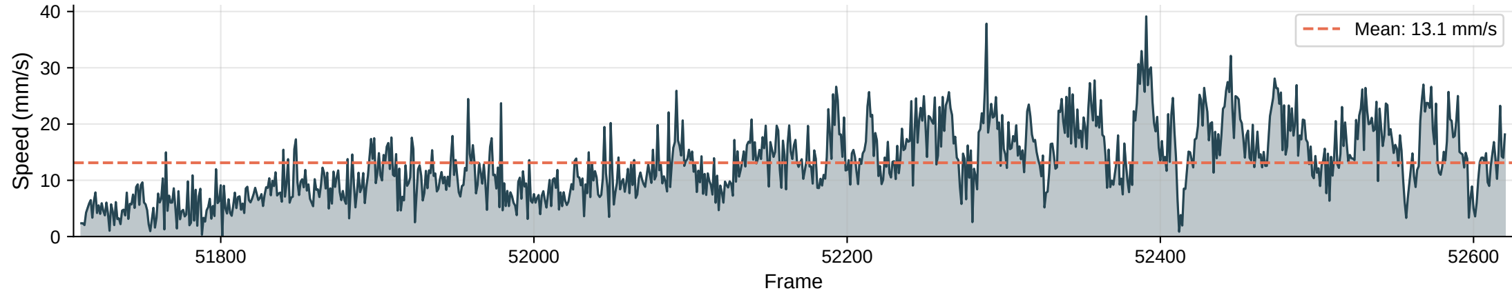
Instantaneous Speed | Max: 39.1 mm/s
