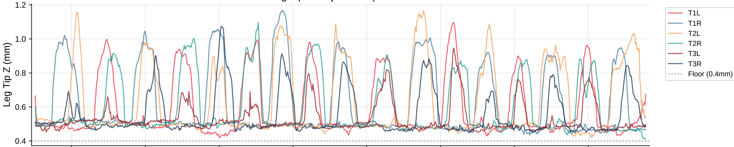
Leg Tip Z Trajectories | Bout 10
