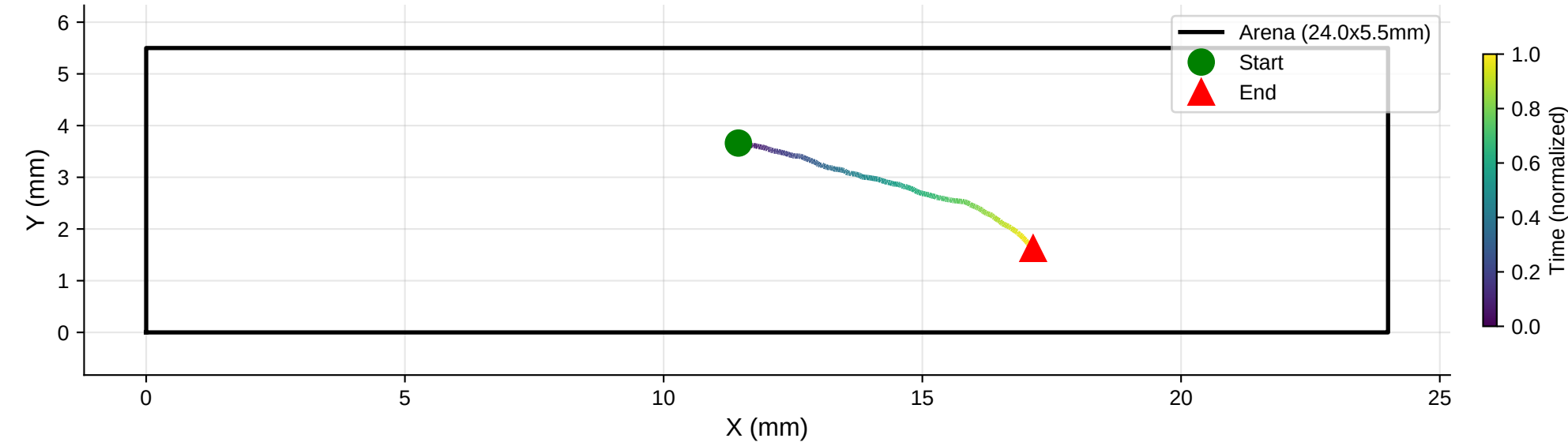
XY Trajectory | Distance: 6.33 mm
