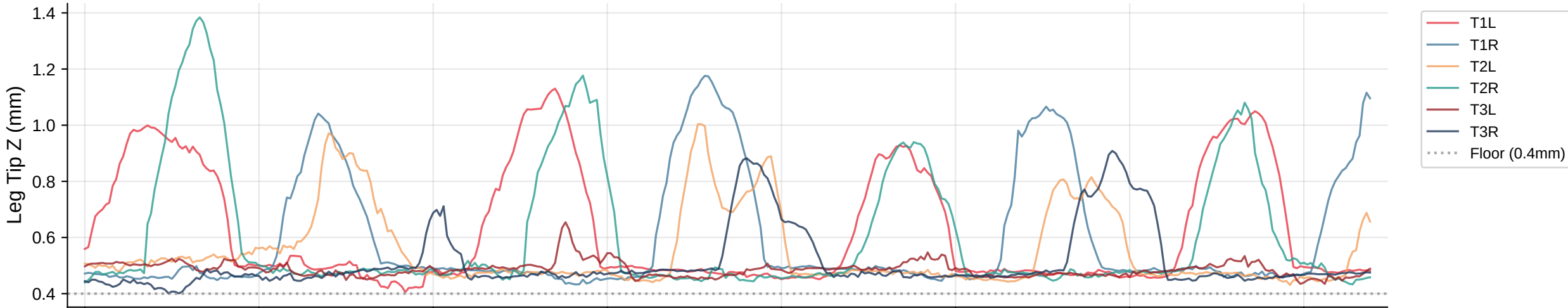
Leg Tip Z Trajectories | Bout 13
