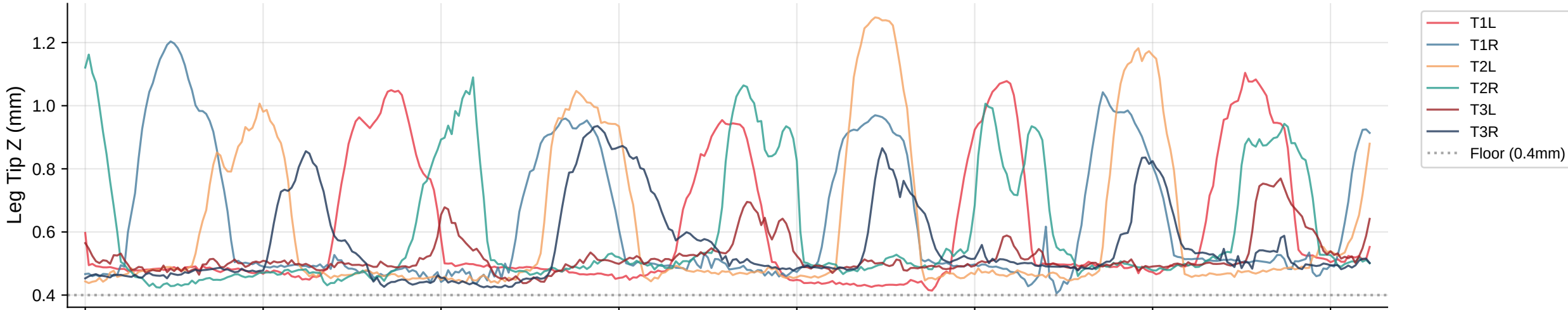
Leg Tip Z Trajectories | Bout 14
