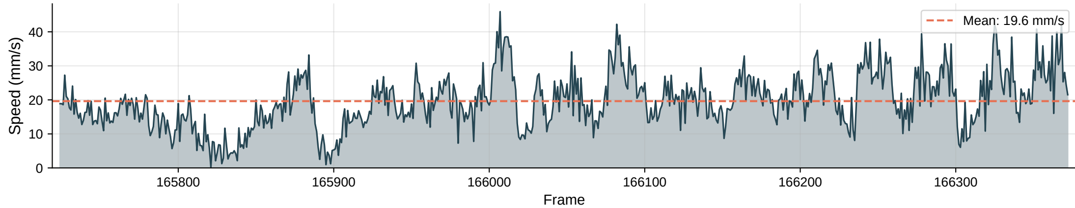
Instantaneous Speed | Max: 45.9 mm/s
