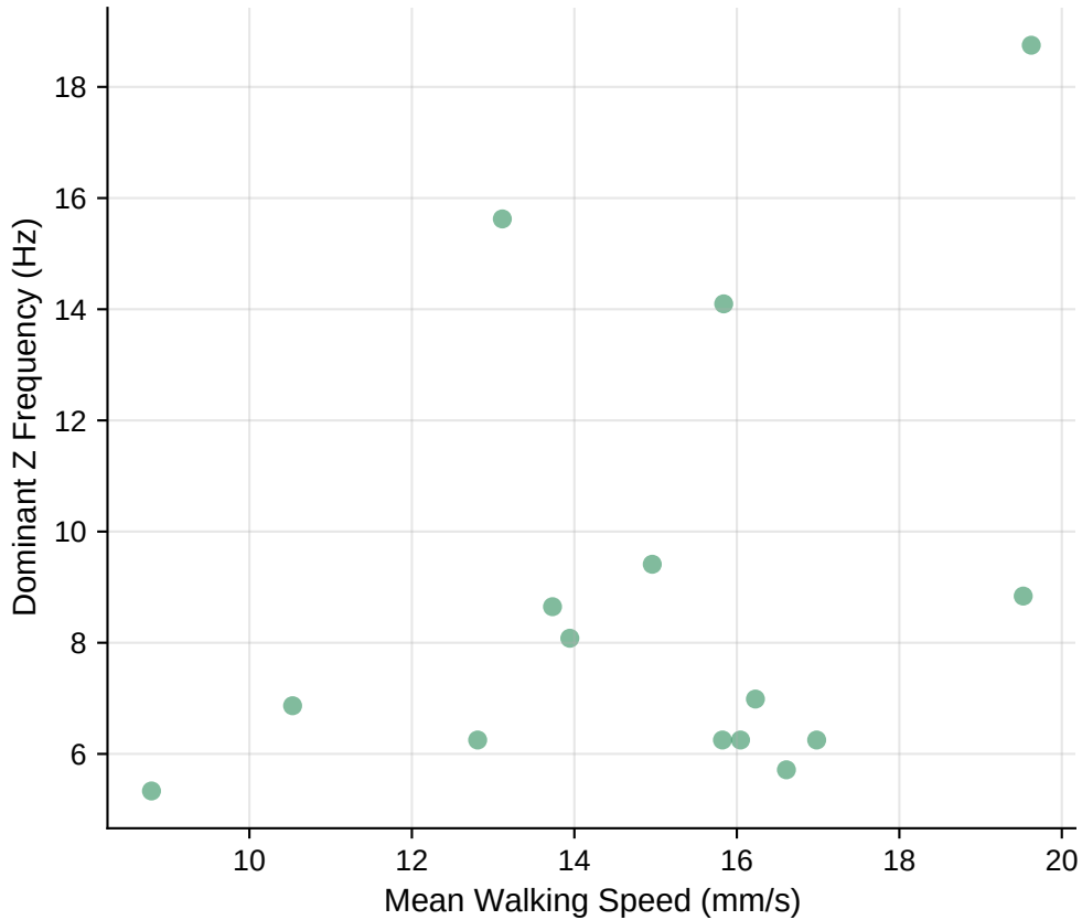
Speed vs Z Oscillation Frequency Pearson r = 0.344 , p = 2.10e-01
