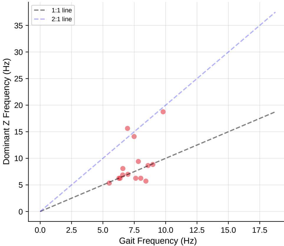
Gait vs Z Frequency Pearson r = 0.473 , p = 7.53e-02
