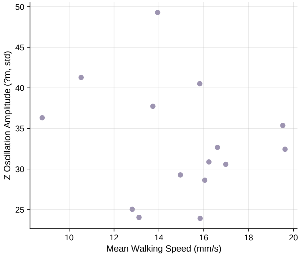
Speed vs Z Oscillation Pearson r = -0.178 , p = 5.25e-01
