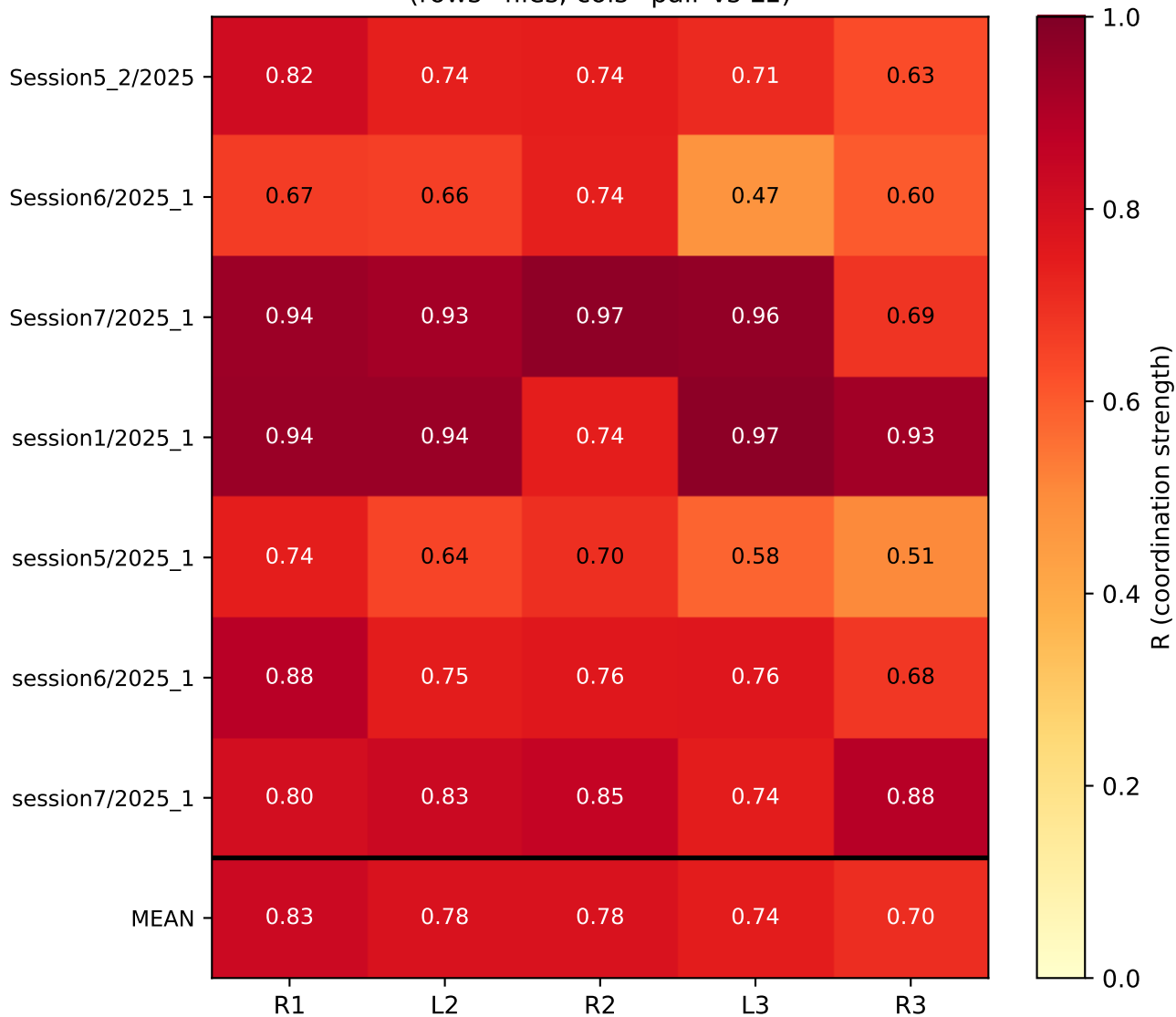
Coordination R Q1 (slowest) [0.0-14.4 mm/s] (rows=flies, cols=pair vs L1)
