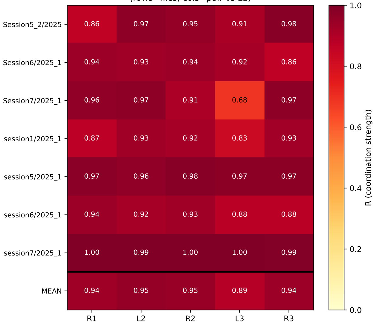
Coordination R Q3 [22.8- \infty mm/s] (rows=flies, cols=pair vs L1)
