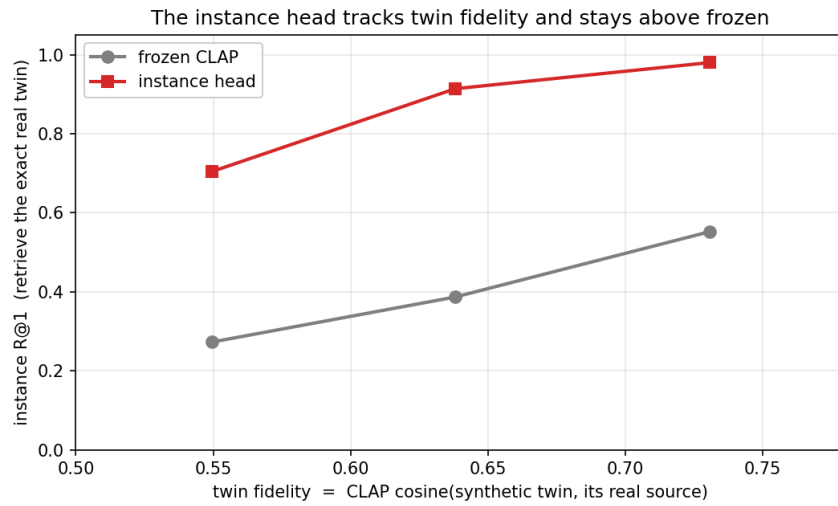
Figure 3: The instance head is not just matching near-copies (fidelity sweep).
