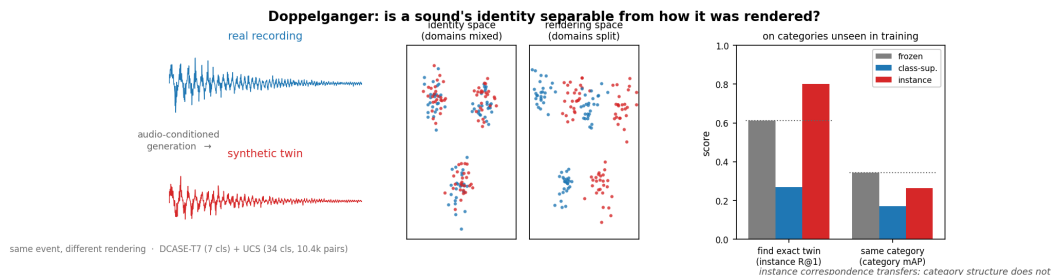
Figure 1: Matching a sound effect to its synthetic twin, and what transfers to unseen sound events.
