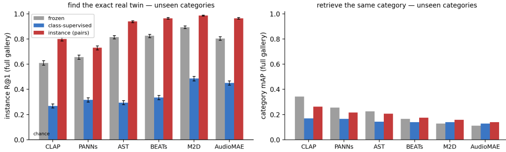
Figure 2: The dissociation holds across six encoders (unseen sound events, full gallery).
