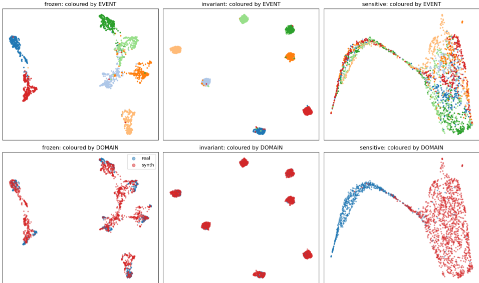
Figure A1: The geometry flips between the invariant and sensitive heads.
