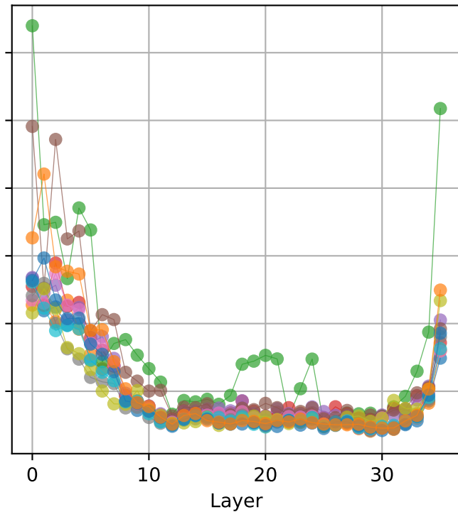
GPT-2 Large
