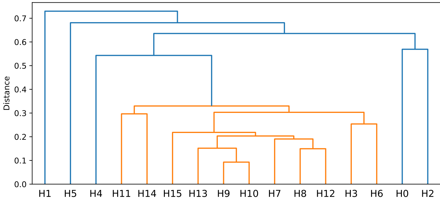
bigscience/bloom-560m: Head Lambda trajectory clustering
