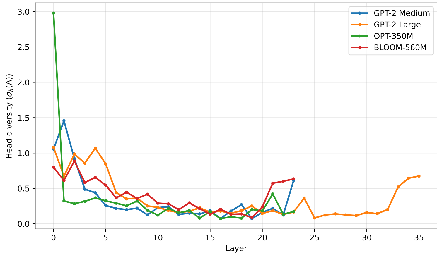
Within-layer Head Diversity of \Lambda
