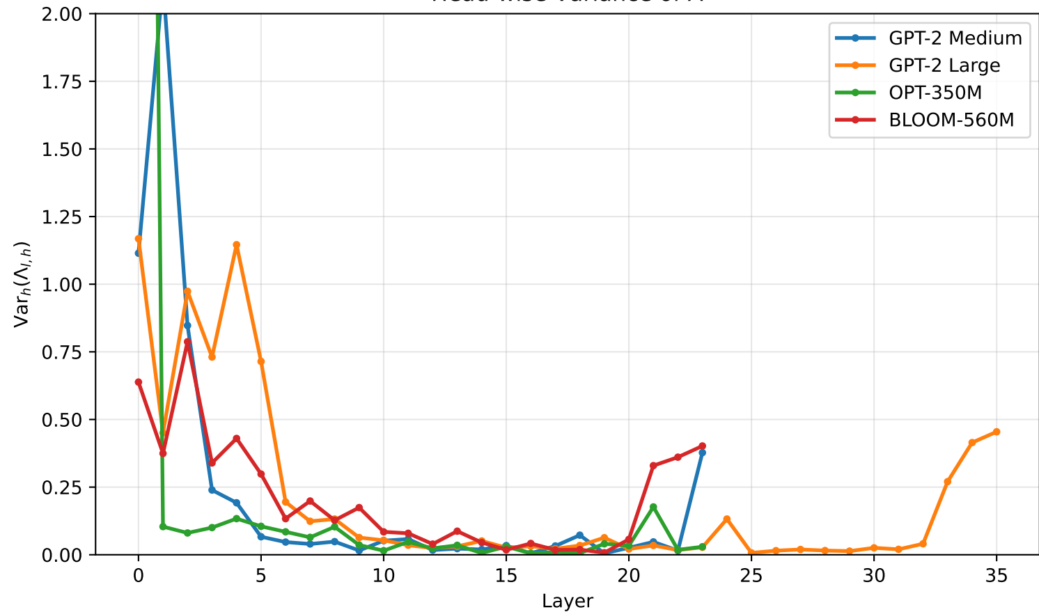
Head-wise Variance of \Lambda
