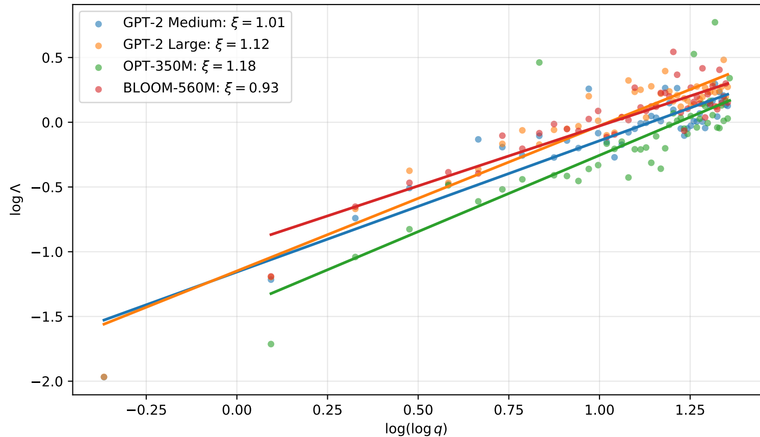
Log-log scaling: \log \Lambda = \xi \log(\log q) + c
