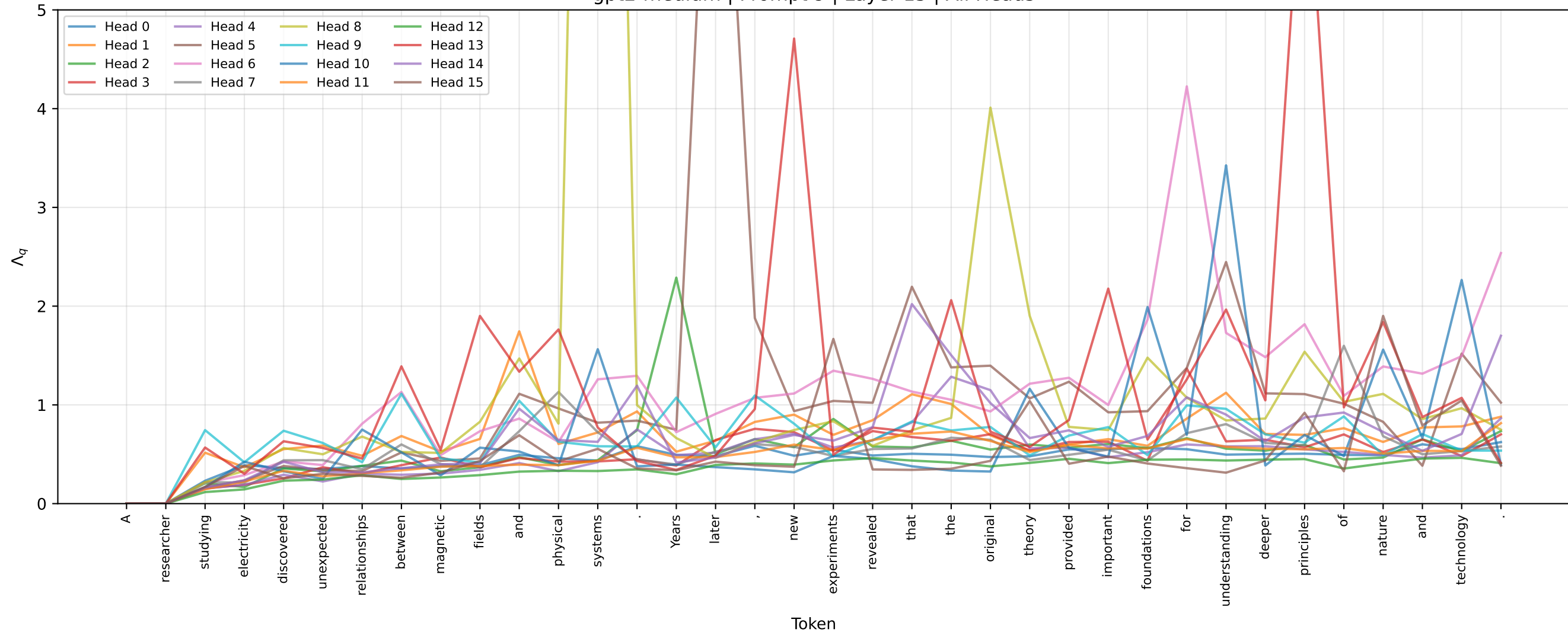
gpt2-medium | Prompt 9 | Layer 15 | All Heads
