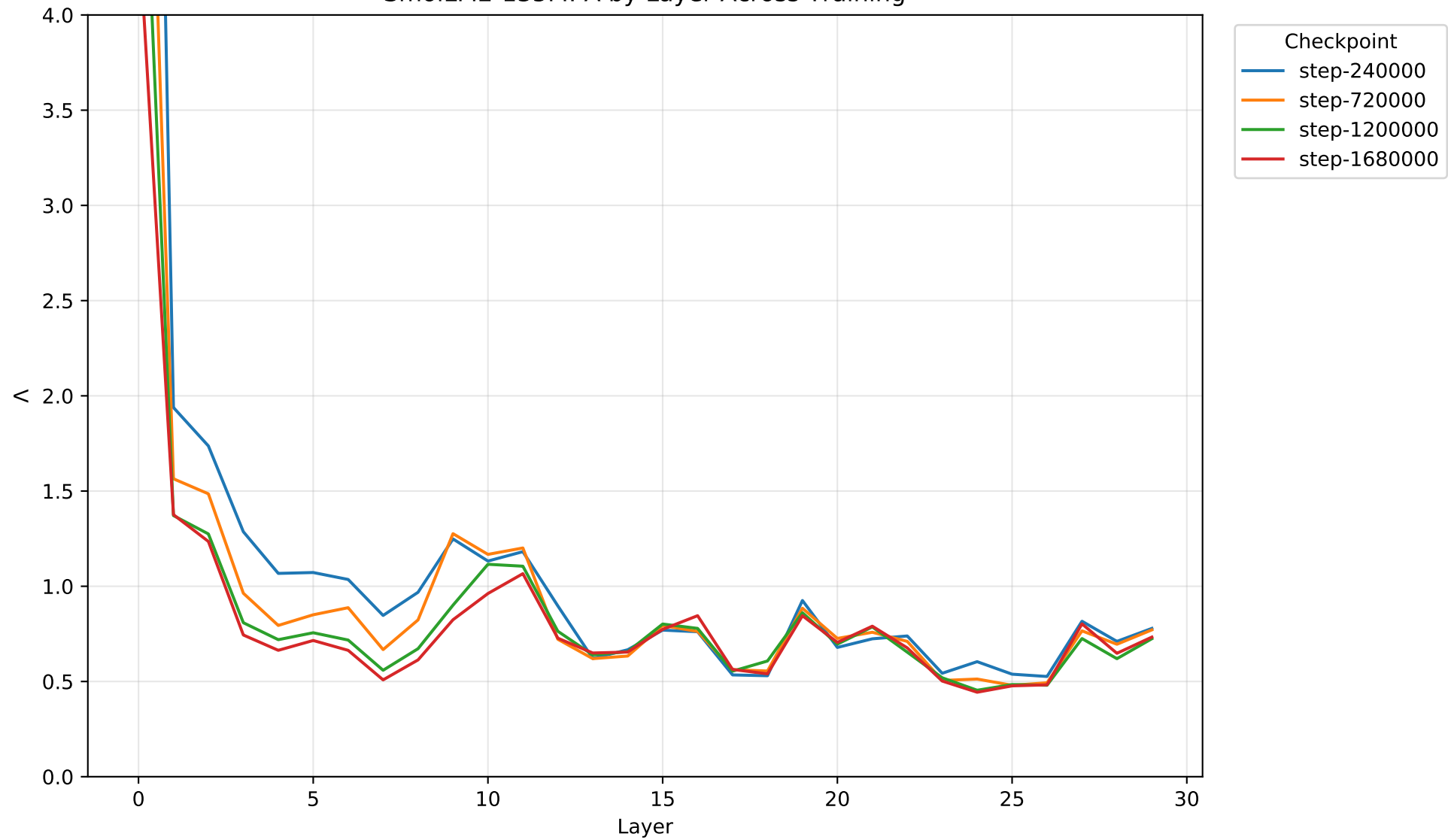
SmolLM2-135M: \Lambda by Layer Across Training
