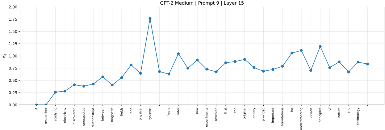
Figure 11: Mean \Lambda over Layer 15 Heads on Prompt 9, GPT-2 Medium.
