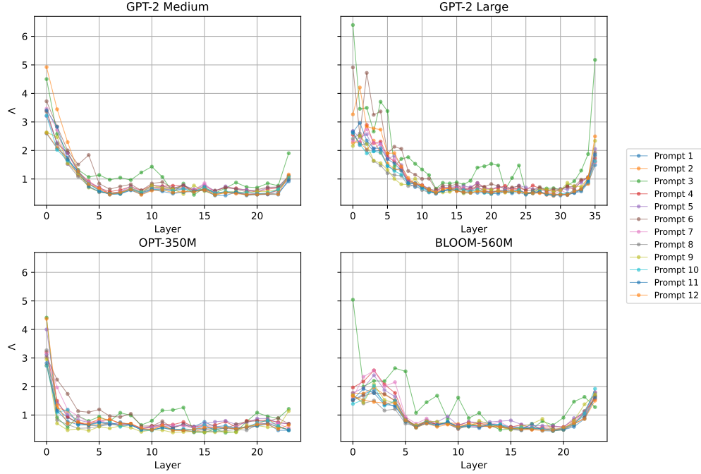
Figure 9: Mean \Lambda by layer and prompt.
