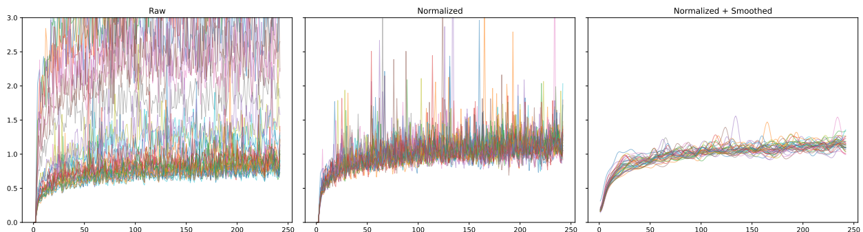
Figure 12: Normalization and smoothing on prompt-averaged \Lambda_{l,i} , GPT2-Large.
