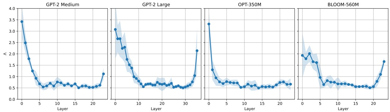
Figure 8: Evolution of mean \Lambda by layer. Shaded regions show \pm 1 std across prompts.
