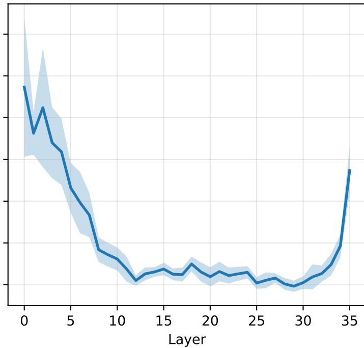
GPT-2 Large
