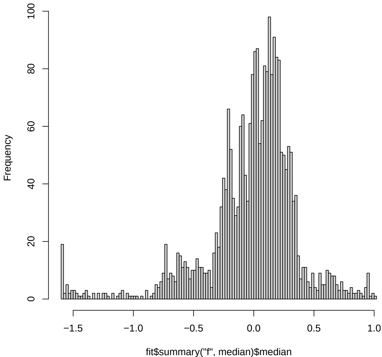
Histogram of fit$summary("f", median)$median
