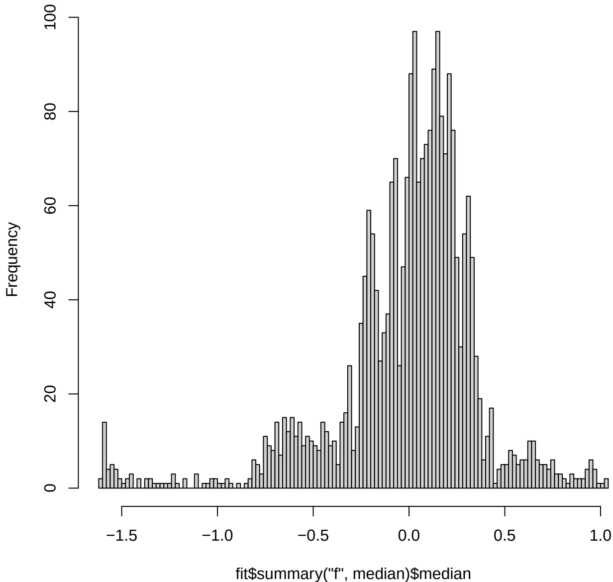
Histogram of fit$summary("f", median)$median
