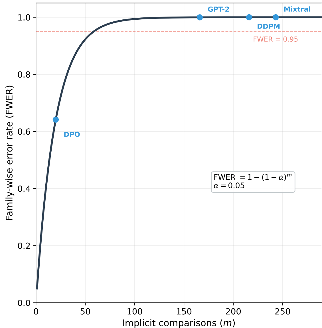
FWER curve
