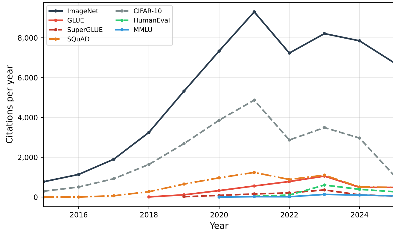
(a) Benchmark adoption and abandonment
