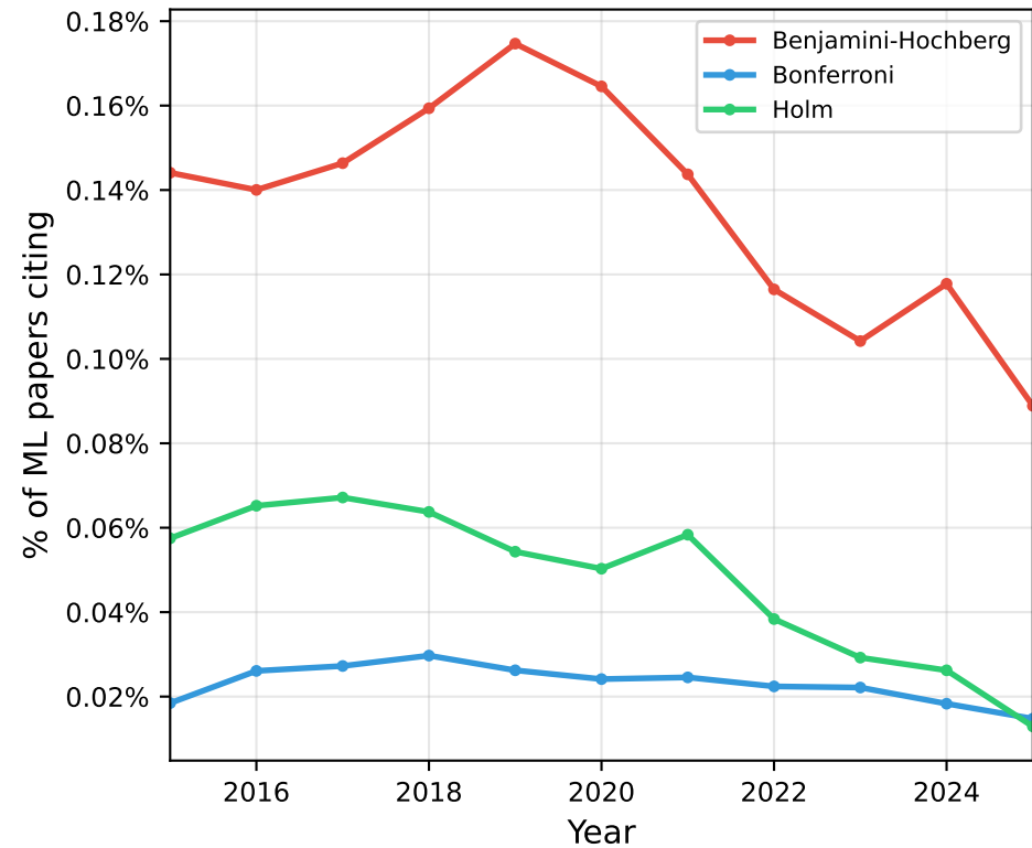
(b) Statistical correction adoption
