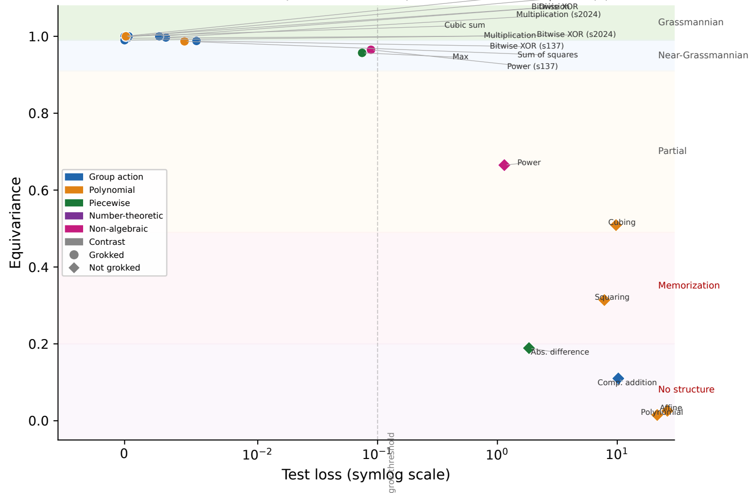
Test loss vs equivariance — all operations and seeds
