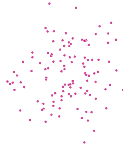
affine (s42) eq=0.026, CV=0.46
