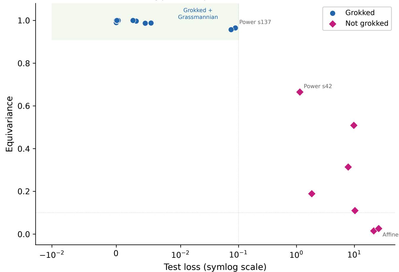
Grokking predicts equivariant causal structure
