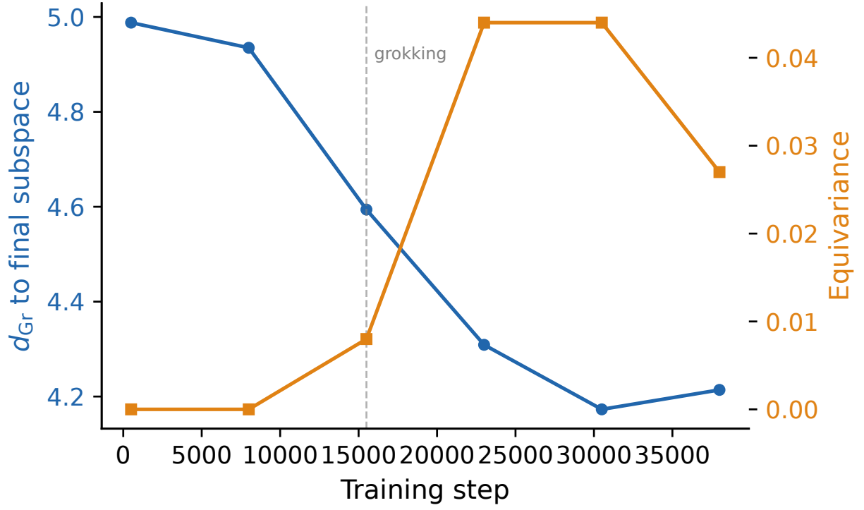
Figure 7: Grassmannian trajectory during grokking for modular multiplication. The Grassmannian distance d_{Gr} from the current DAS subspace to the final (fully grokked) subspace decreases as equivariance rises. The subspace converges to its final position during the grokking phase transition (dashed line), confirming that spectral compression and causal structure emerge simultaneously.
