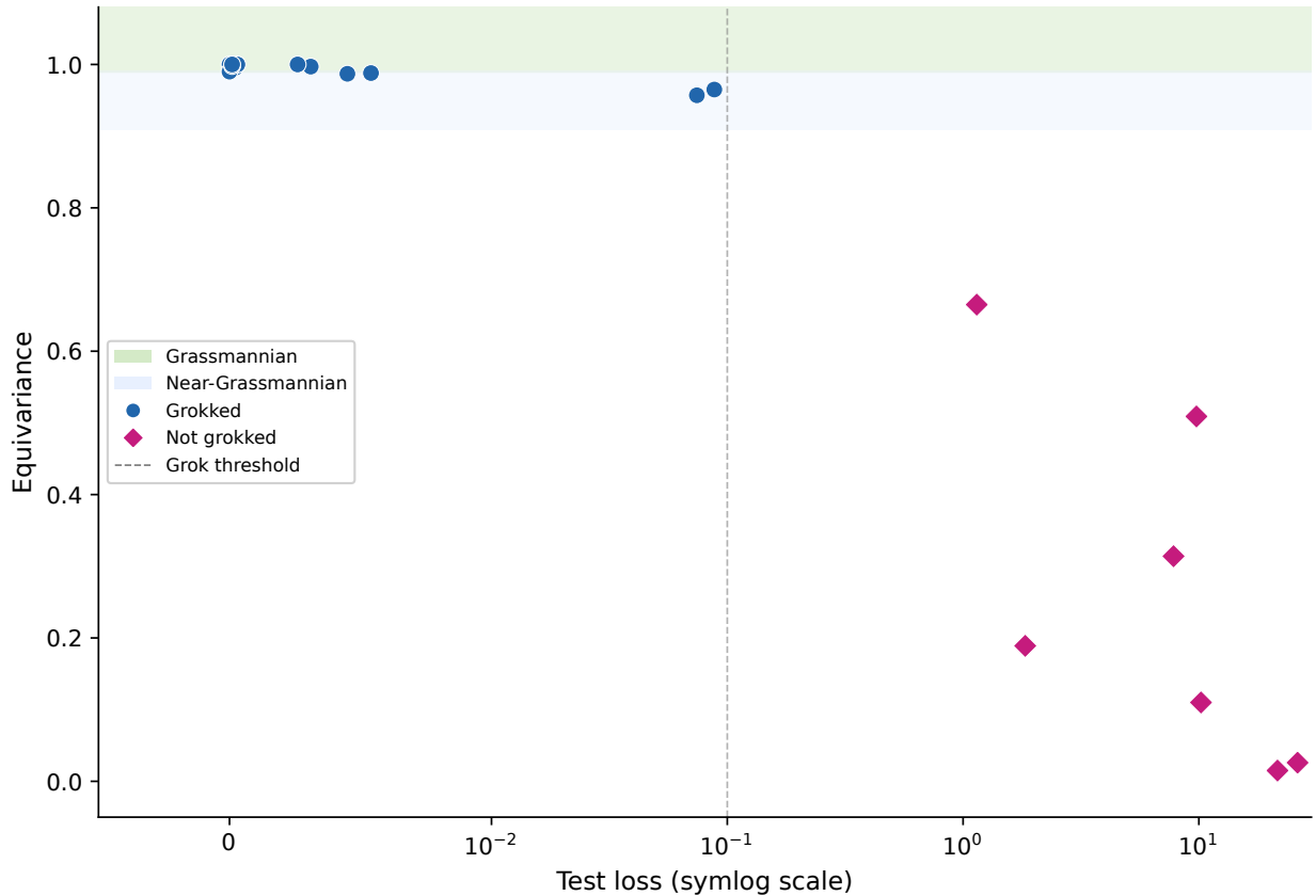
Figure 3: Test loss vs. equivariance across all operation–seed pairs. The dashed line marks the grokking threshold (test loss = 0.1). Grokked operations (blue, left of threshold) achieve equivariance > 0.95 ; non-grokked operations (pink, right) scatter across the full range. The separation is sharp: no operation crosses the threshold with intermediate equivariance.
