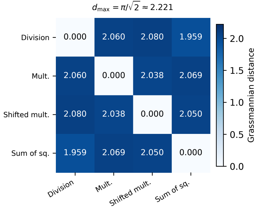
Figure 6: Pairwise Grassmannian distances between DAS subspaces fitted to four grokked operations. All distances cluster near d_{\max} = \pi/\sqrt{2} \approx 2.22 radians, indicating near-orthogonal subspaces. Each operation learns a valid causal variable, but these variables occupy different regions of \text{Gr}(2, 128) .
