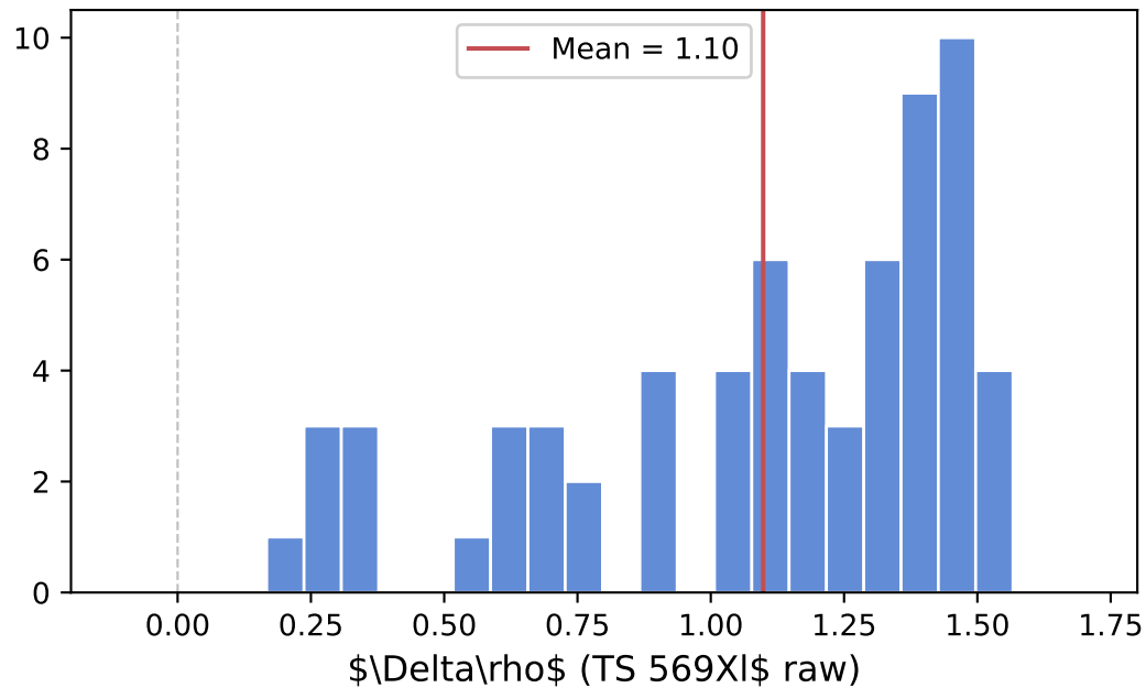
All 66 folds: \Delta\rho > 0
