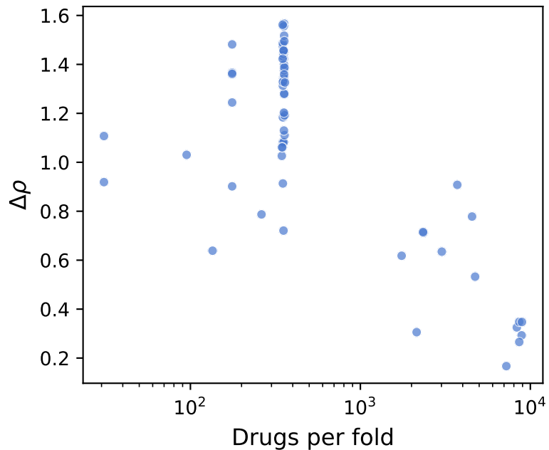
Frequency gradient \rho = -0.32 , p = 0.009
