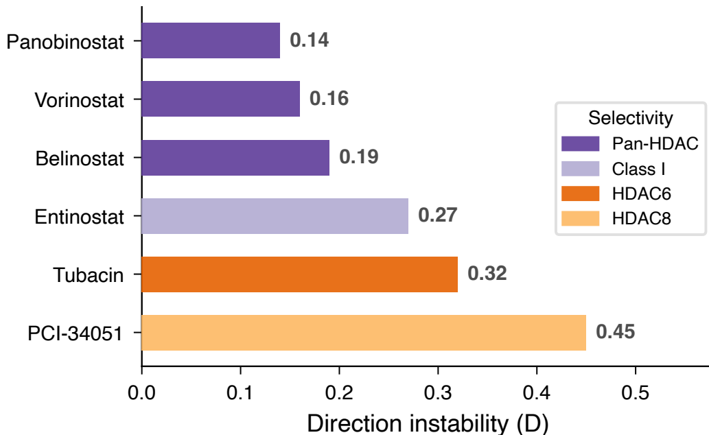
Figure 1: HDAC selectivity gradient: calibration standard for direction instability. Pan-HDAC inhibitors [8] (panobinostat, vorinostat, belinostat) achieve the lowest direction instability ( D = 0.14 – 0.19 ); Class I-selective entinostat is intermediate ( D = 0.27 ); isoform-selective HDAC6 and HDAC8 inhibitors (tubacin, PCI-34051 [9]) have the highest instability within the class ( D = 0.32 – 0.45 ). This gradient, reproduced from Tower [6], provides a fine-grained rank ordering within the HDAC class: Spearman \rho = 0.83 between direction instability and selectivity rank across these 6 compounds after toxicity-gene correction. The HP1 “doesn’t bite” threshold ( \rho \geq 0.83 ) was calibrated to this value.
