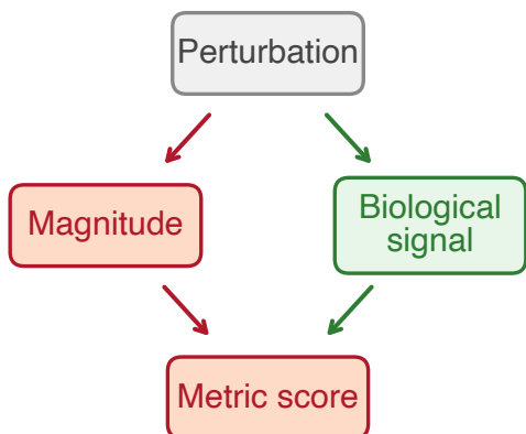
Figure 1: Direction instability removes linear magnitude dependence. (a) Confounded metrics (variance, subspace size) inherit effect magnitude through a shared path, producing spurious associations between perturbation strength and metric value. (b) Direction instability operates after cosine normalization, which blocks the linear magnitude path under the assumption that signature direction is independent of dose (separability). The observed association between group variable and metric reflects biological signal to the extent that this assumption holds. An empirical test of separability (dose-direction stability across 1,445 drugs) is reported in the Discussion.
