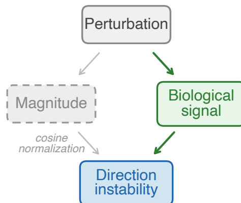
Figure 1: Direction instability removes linear magnitude dependence. (a) Confounded metrics (variance, subspace size) inherit effect magnitude through a shared path, producing spurious associations between perturbation strength and metric value. (b) Direction instability operates after cosine normalization, which blocks the linear magnitude path under the assumption that signature direction is independent of dose (separability). The observed association between group variable and metric reflects biological signal to the extent that this assumption holds. An empirical test of separability (dose-direction stability across 1,445 drugs) is reported in the Discussion.
