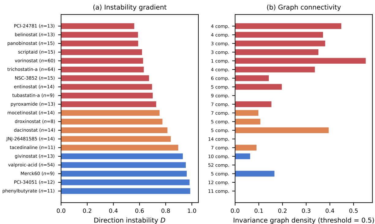
Figure 2: HDAC inhibitor selectivity gradient. (a) Direction instability for all 20 HDAC inhibitors, ordered by D . Pan-isoform inhibitors (red) cluster at low instability; selective and weak inhibitors (blue) are indistinguishable from the population. (b) Invariance graph density at cosine threshold 0.5 and number of connected components. Pan-inhibitors form few components (dense graphs); selective inhibitors fragment into isolated nodes.
