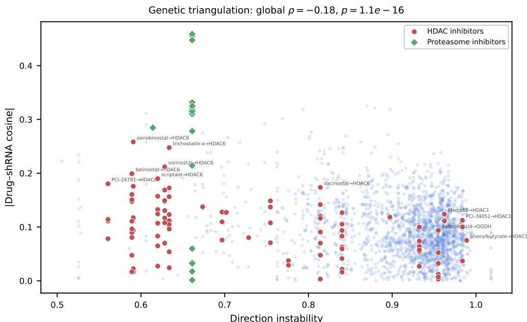
Figure 4: Genetic triangulation: direction instability versus |drug-shRNA cosine| for 2,138 drug-target pairs. HDAC inhibitors (red circles) and proteasome inhibitors (green diamonds) are highlighted. Proteasome inhibitors cluster at high cosine and low instability; HDAC inhibitors span the full gradient. Labels show drug-target pairs for selected HDAC inhibitors. The global correlation ( \rho = -0.18 ) is attenuated by cross-family baseline differences (proteasome cos \approx 0.45 vs. HDAC cos \approx 0.15 ); within-family stratification yields |\rho| = 0.32\text{--}0.84 (Table 2).
