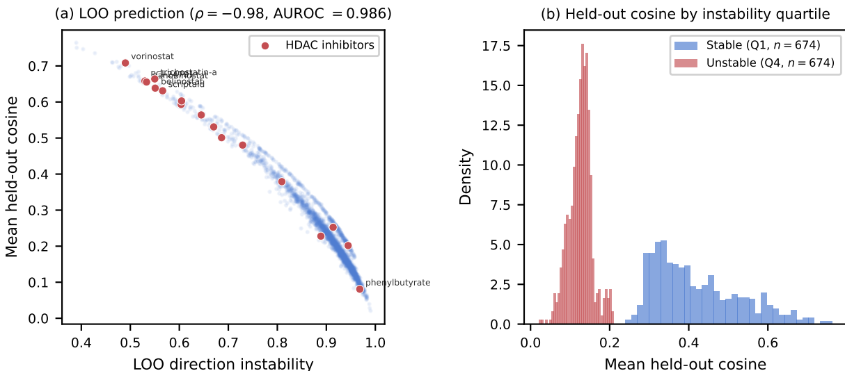
Figure 5: Held-out prediction of drug mechanism transport. (a) Direction instability computed on N-1 cell lines (x-axis) versus mean cosine between the held-out signature and the N-1 consensus (y-axis), for 2,694 drugs with \geq 10 cell lines. Red points are HDAC inhibitors. The tight curve ( \rho = -0.98 , AUROC = 0.986) shows that instability predicts held-out consistency, not merely correlates with it. (b) Histogram of held-out cosine for the most stable (Q1, blue) and least stable (Q4, red) quartiles. The distributions barely overlap: stable drugs reliably transport to new contexts.
