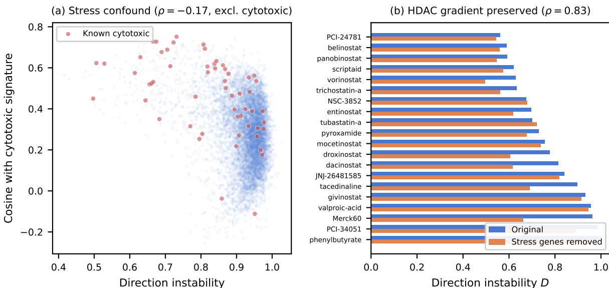
Figure 3: Cytotoxicity confound check. (a) Direction instability versus cosine similarity with the mean cytotoxic signature ( \rho = -0.17 , excluding known cytotoxic drugs in red). The negative sign rules out the confound: drugs resembling the stress response are less stable, not more. (b) HDAC inhibitor instability before (blue) and after (orange) removing 50 stress-associated genes. The selectivity gradient is preserved ( \rho = 0.83 ), and pan-inhibitors become more stable.
