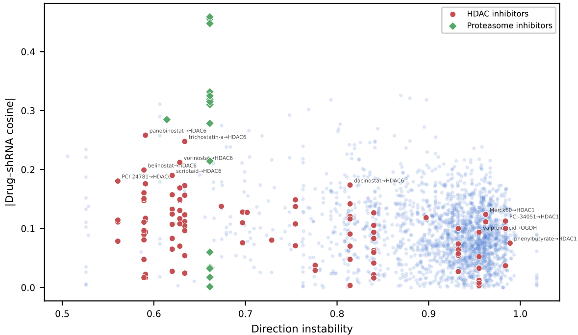
Genetic triangulation: global \rho = -0.18 , p = 1.1e-16
