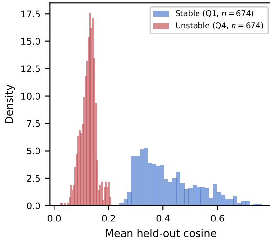
(b) Held-out cosine by instability quartile
